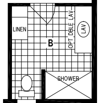
7333MB/6628 (1,782 SQ. FT.) 3BEDROOM - 2BATHS
